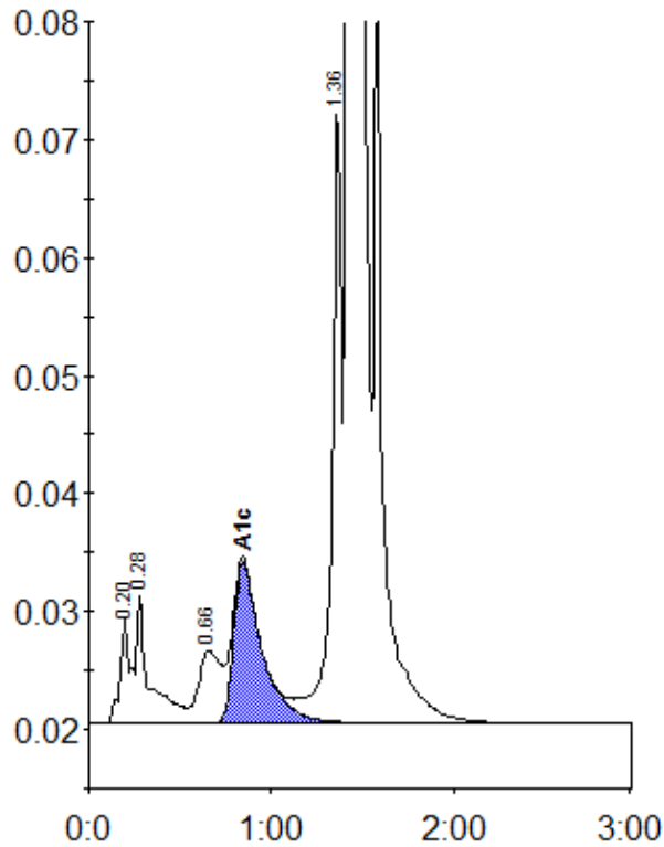
Peak table - ID: 10344810
